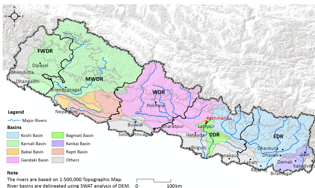
Figure 3: River basin and drainage of Nepal
